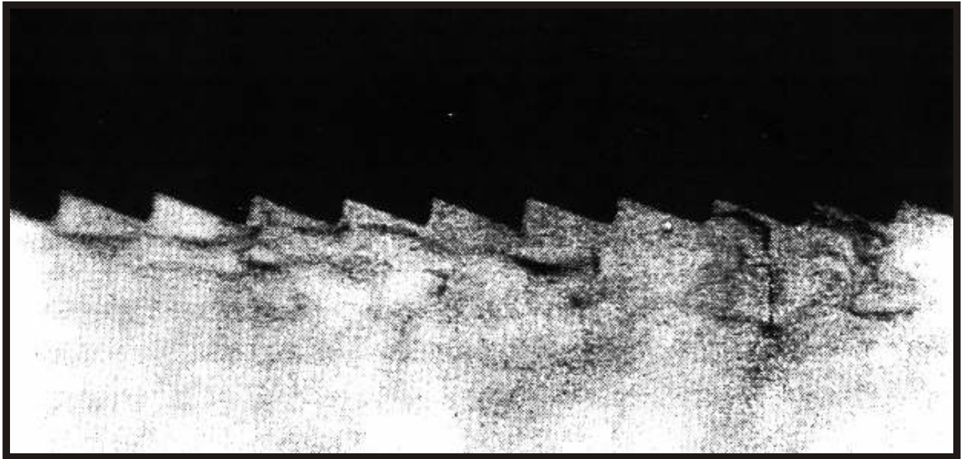
Blazed Gratings etched in Ge (OPT Application lab)
